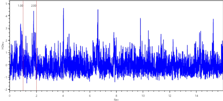
Time Signal
