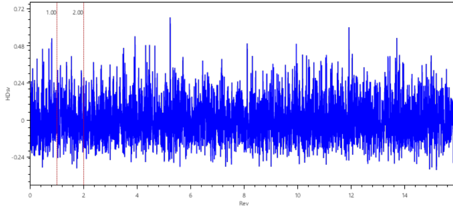
Time Signal
