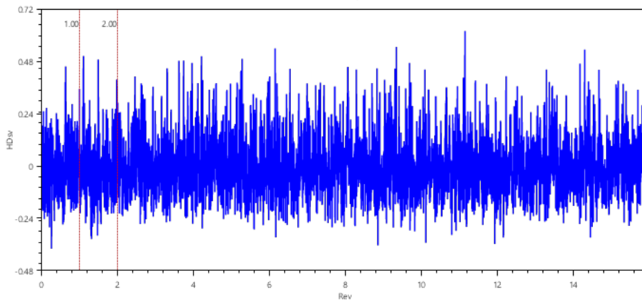
Time Signal
