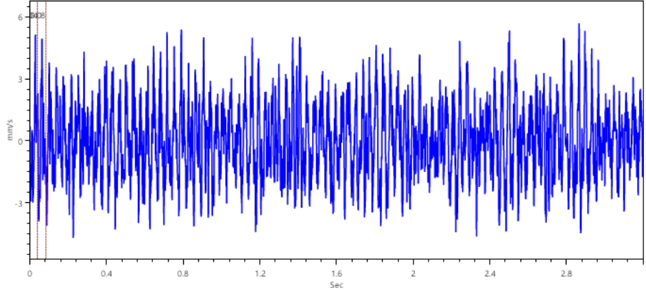
Time Signal
