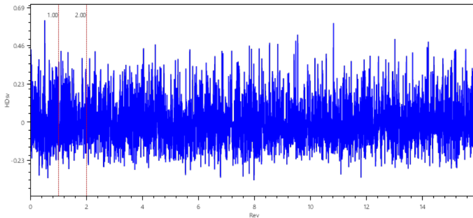
Time Signal
