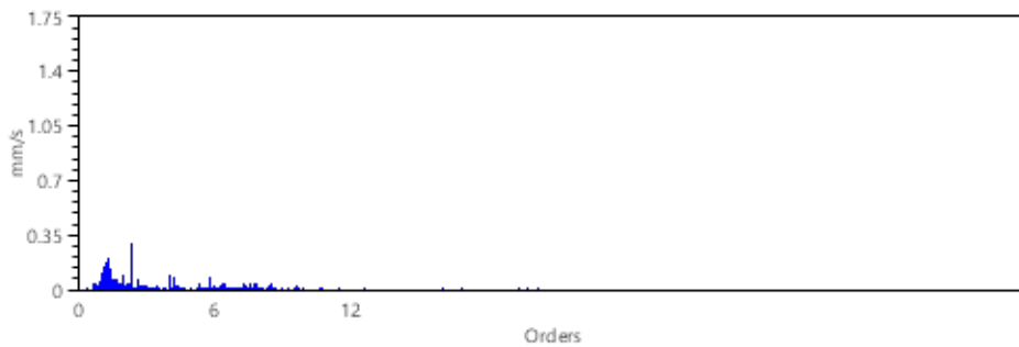
Spectrum
