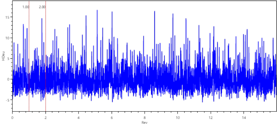
Time Signal
