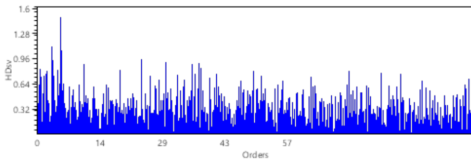
Spectrum
