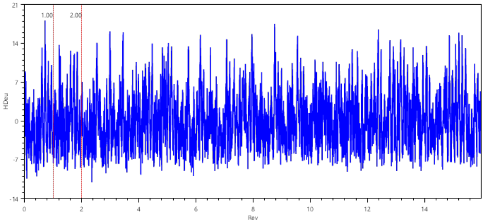
Time Signal
