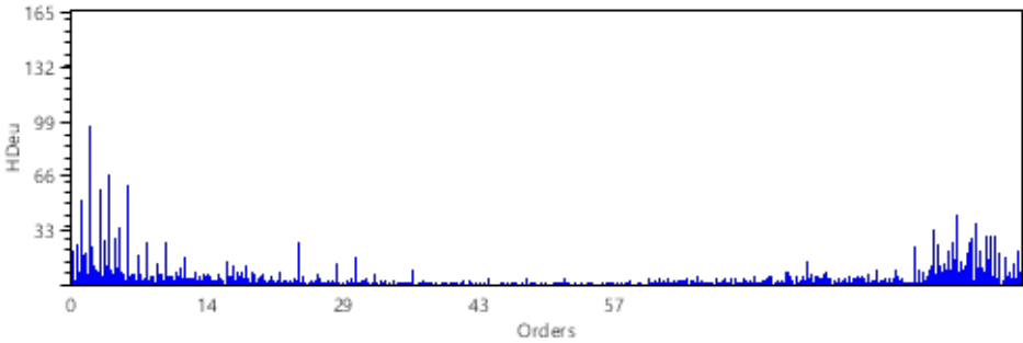
Spectrum
