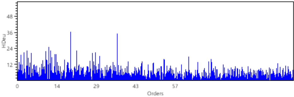
Spectrum
