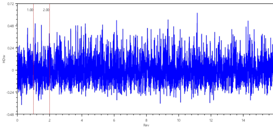
Time Signal
