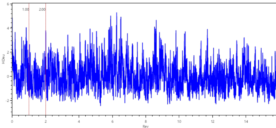
Time Signal
