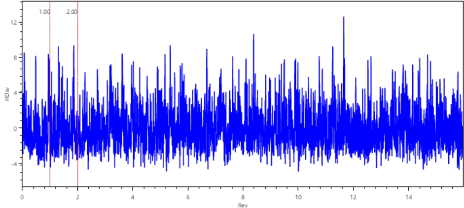
Time Signal
