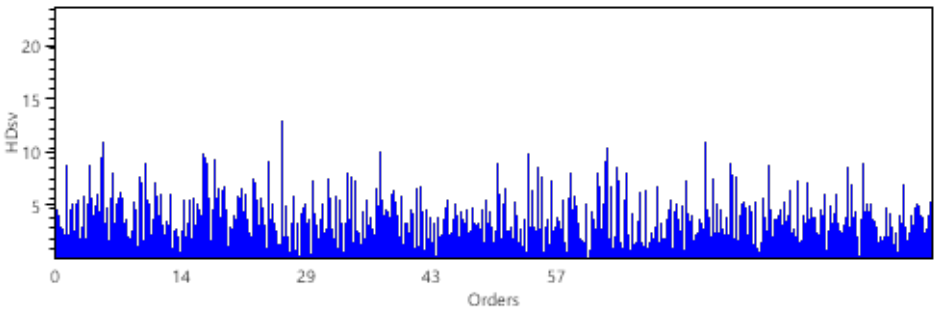
Spectrum
