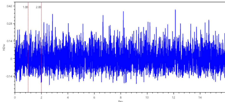
Time Signal
