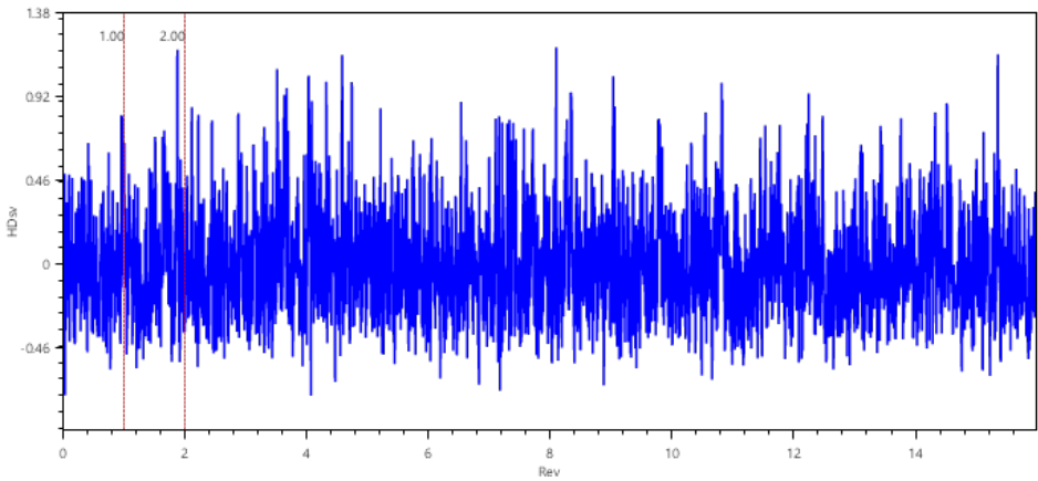
Time Signal
