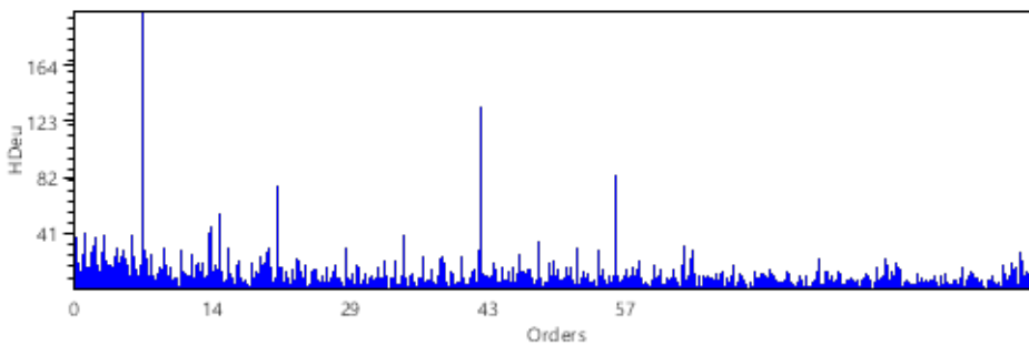
Spectrum
