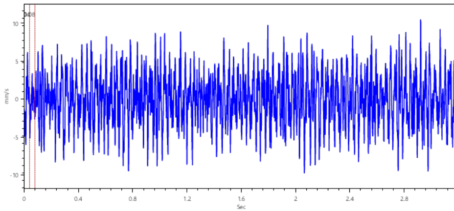
Time Signal
