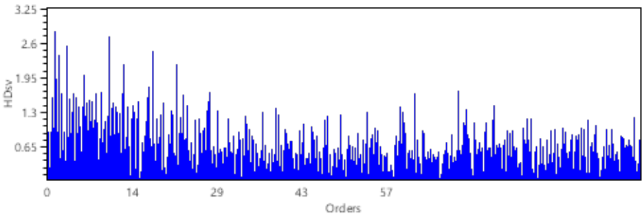
Spectrum
