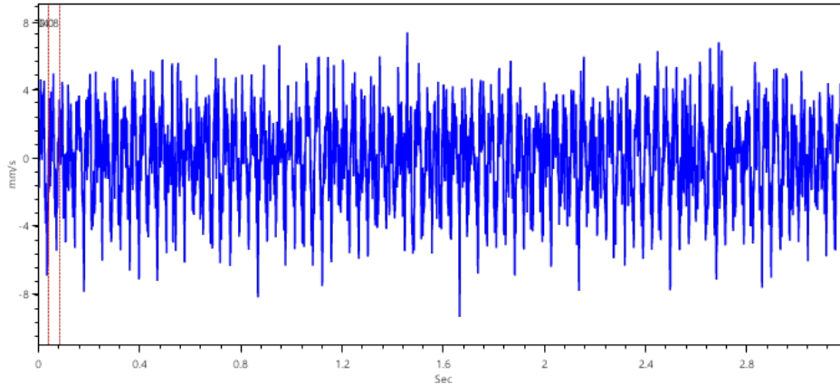
Time Signal
