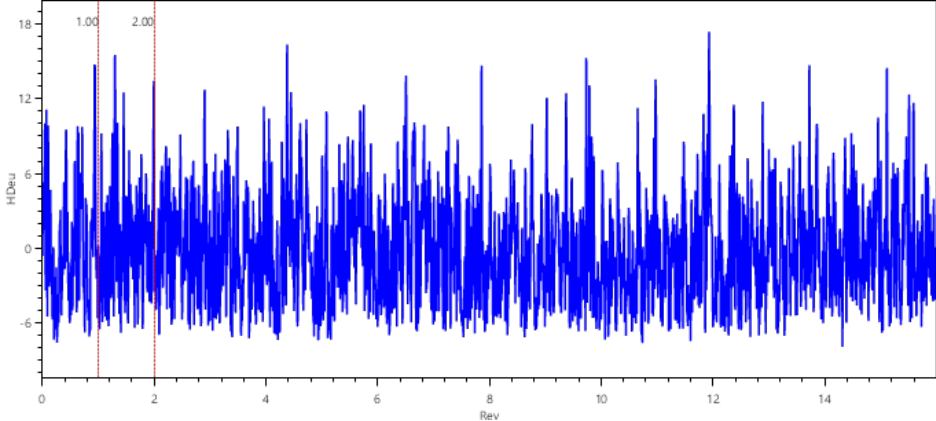
Time Signal
