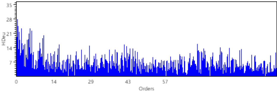
Spectrum
