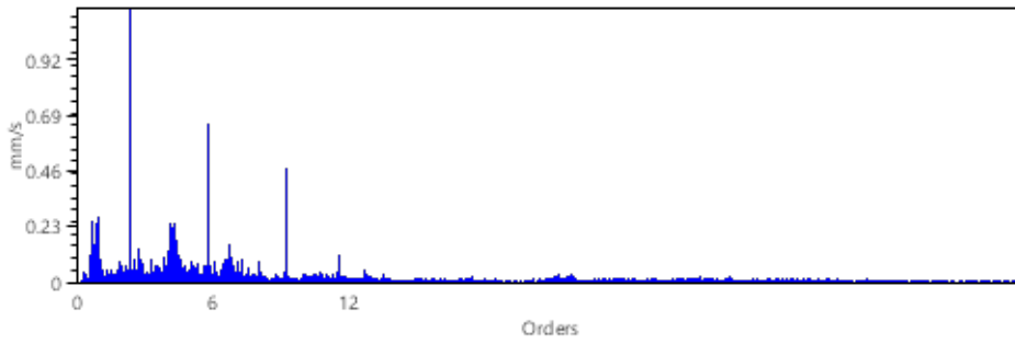
Spectrum
