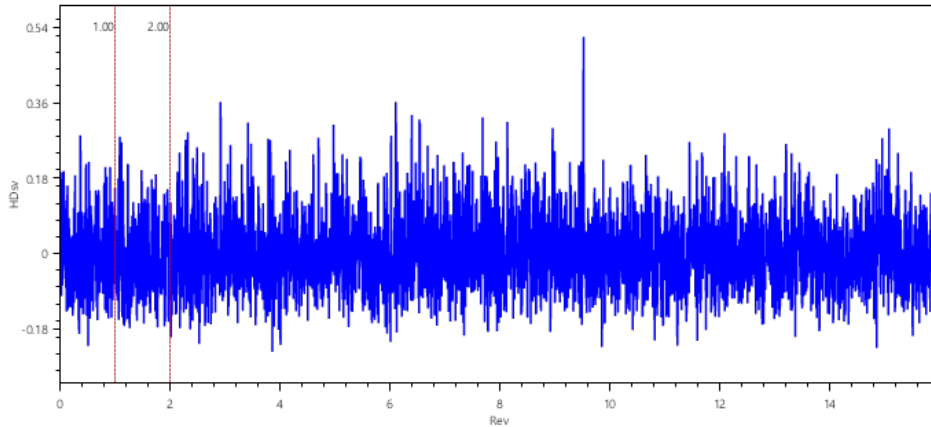
Time Signal
