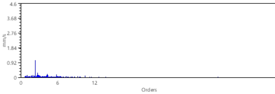
Spectrum
