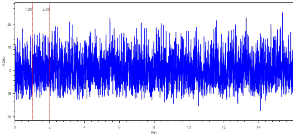
Time Signal
