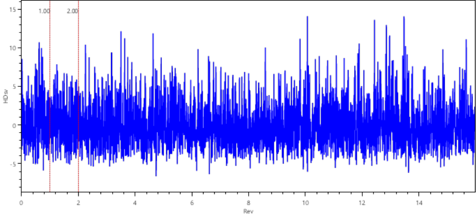
Time Signal
