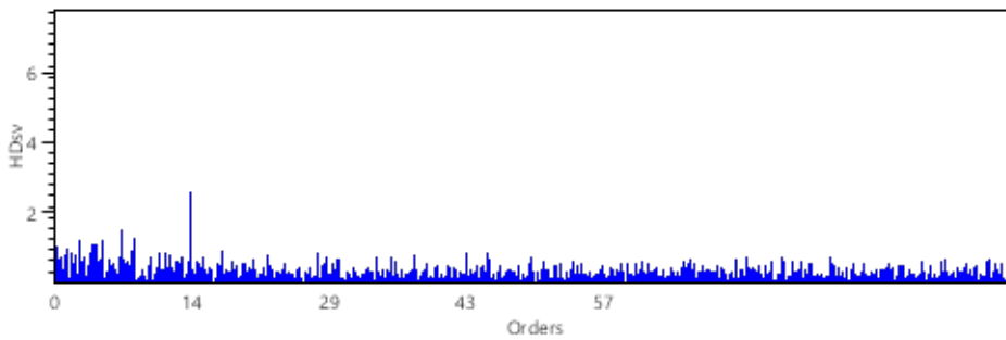
Spectrum
