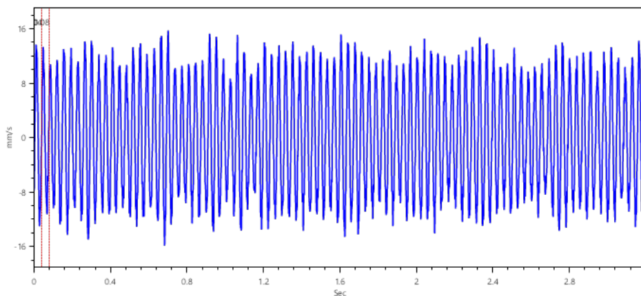
Time Signal
