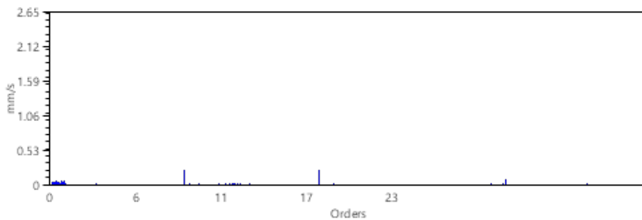
Spectrum
