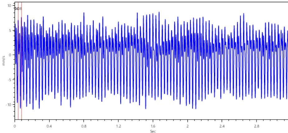
Time Signal
